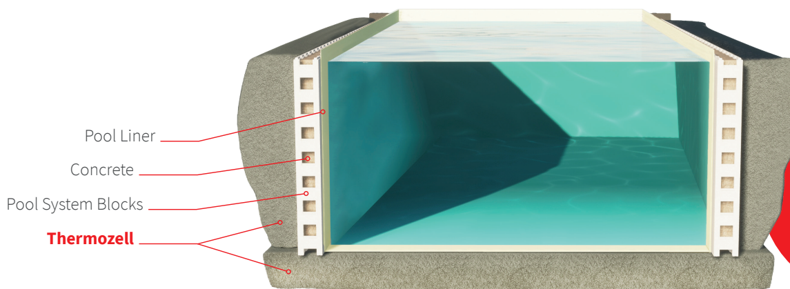
Pool Backfill
